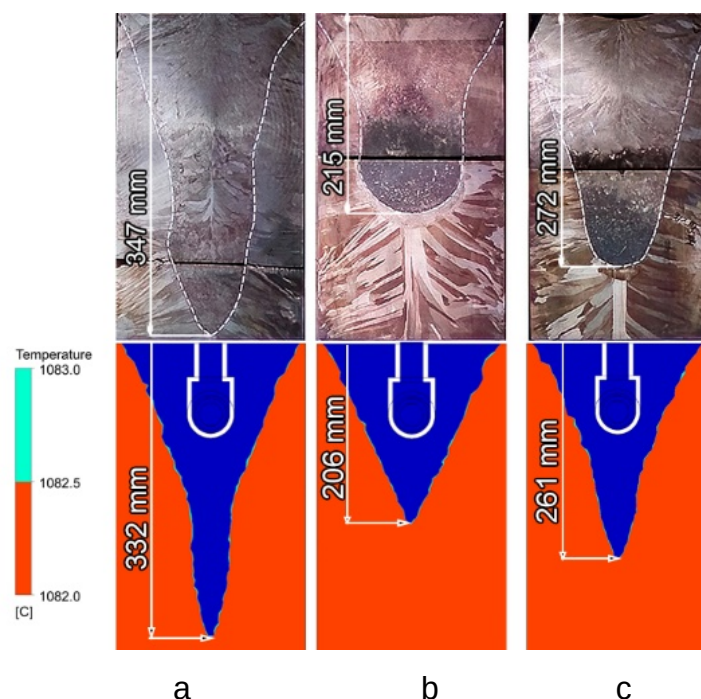
Fig. 3. Comparison of experimental macrostructures (top) and CFD-predicted solidification profiles (bottom) for different submerged entry nozzle configurations: (a) Case 1; (b) Case 2; (c) Case 3.
