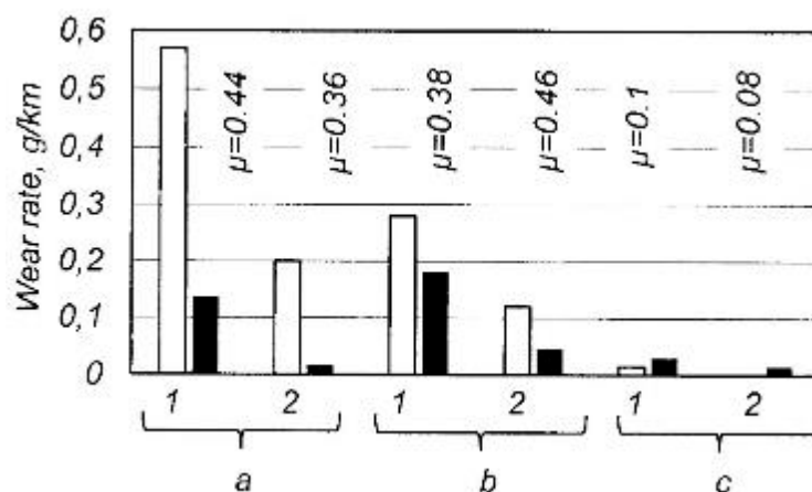
Fig. 3 – Wear rates of the studied Fe-Cr-C (1) and Fe-Cr-Cu-C-Ti (2) alloys in: (a) air; (b) water; (c) oil. □ – specimen, ■ – counterbody.
