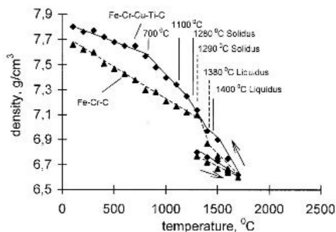
Fig. 1 – Density-temperature curves for the alloys.
