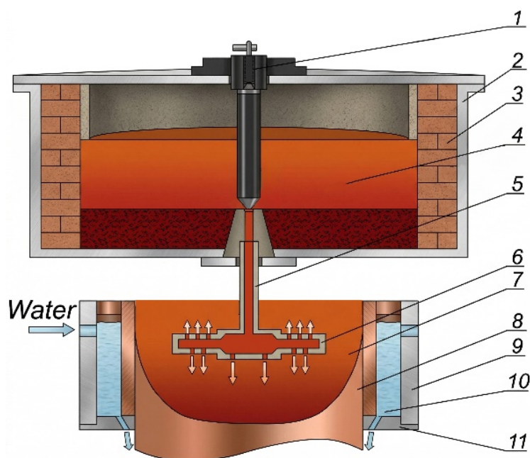
Fig. 1. – Stopper rod casting system for slab caster:
