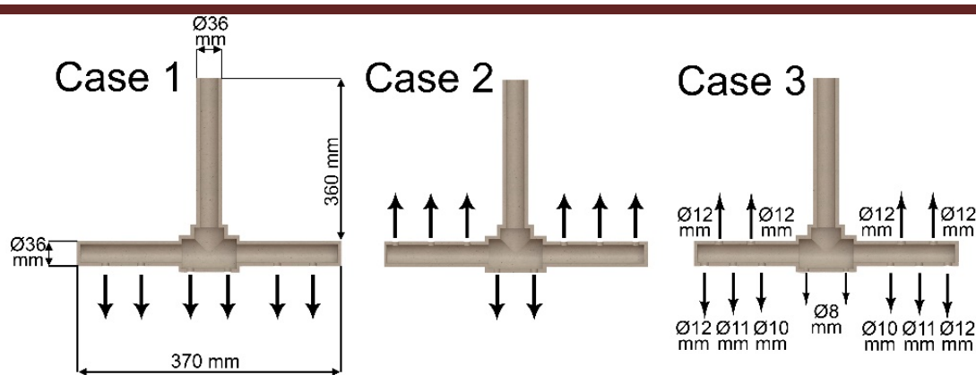
Fig. 2. Geometric configurations of the submerged entry nozzles (SEN) evaluated in the CFD simulations.
