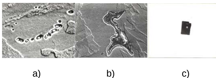
Fig. 1 – Inclusions in 09G2FB and 17G1SU steel samples without yttrium additives: a) – manganese sulfides in 17G1SU steel (x 1100); b) – manganese sulfide in 09G2FB steel (x550); c) – titanium nitride in 09G2FB steel (x5000)
