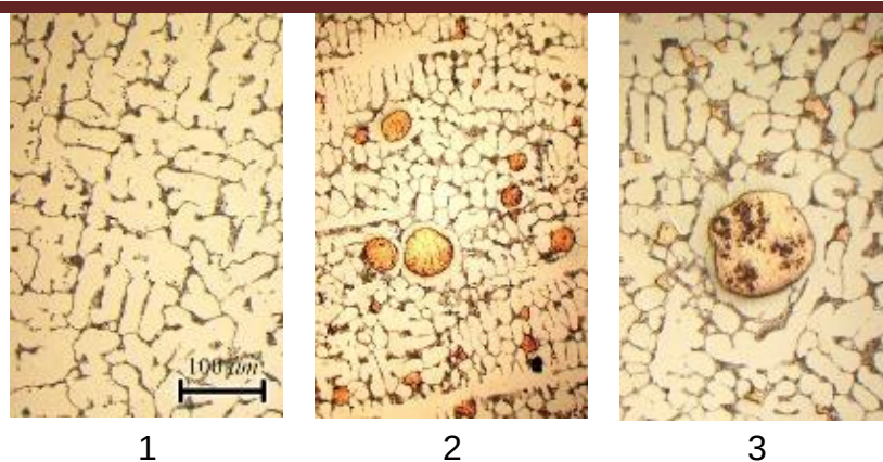
Fig. 2 – Micrographs of the studied Fe-Cr-C (No. 1), Fe-Cr-Cu-Ti-C (No. 2), and Fe-Cr-Cu-V-C (No. 3) alloys.
