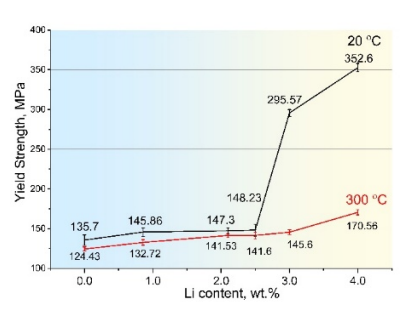
i. Results of compression tests of experimental alloys
