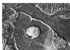
Fig. 3 – Single non-metallic inclusion in 09G2FB steel with 0.08% Y (x5000)
