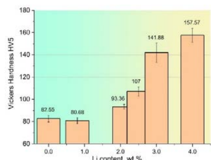
g. Results of HV5 hardness tests
